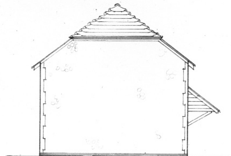
east elevation 1:100
