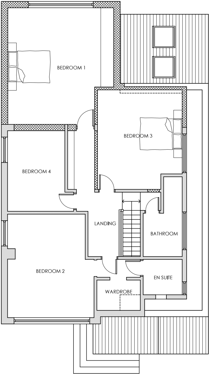
APPROVED FIRST FLOOR PLAN
