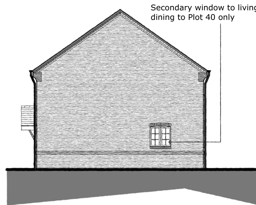
SIDE ELEVATION [1] - 1:100
