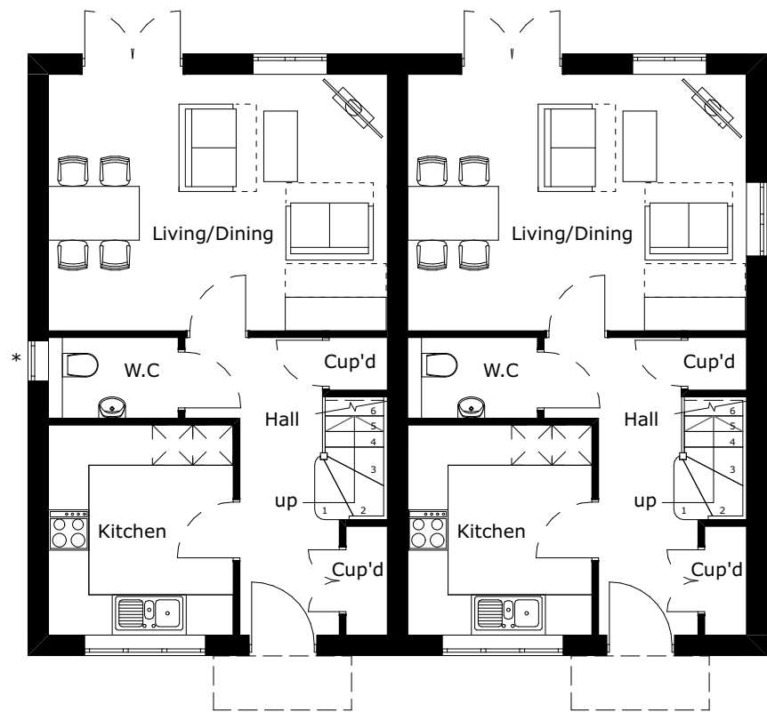
GROUND FLOOR - 1:100
