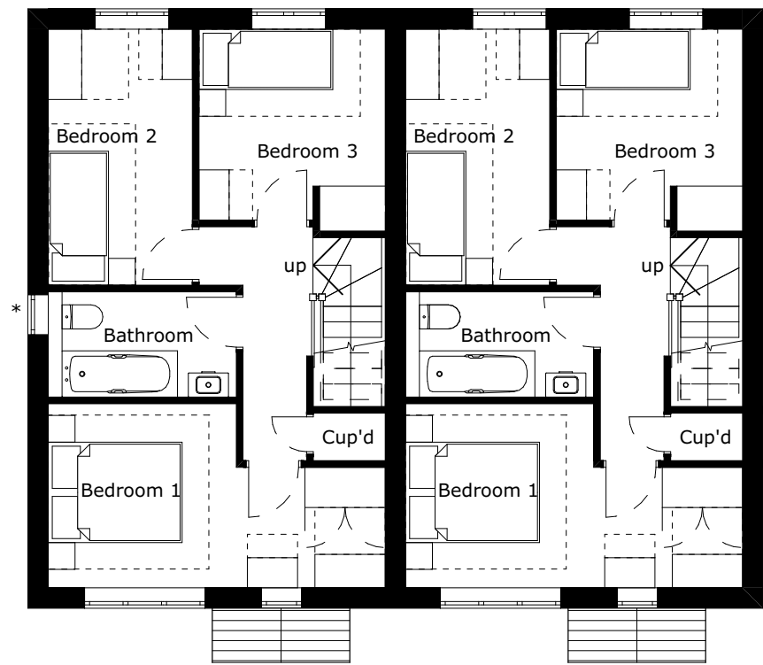
FIRST FLOOR - 1:100
