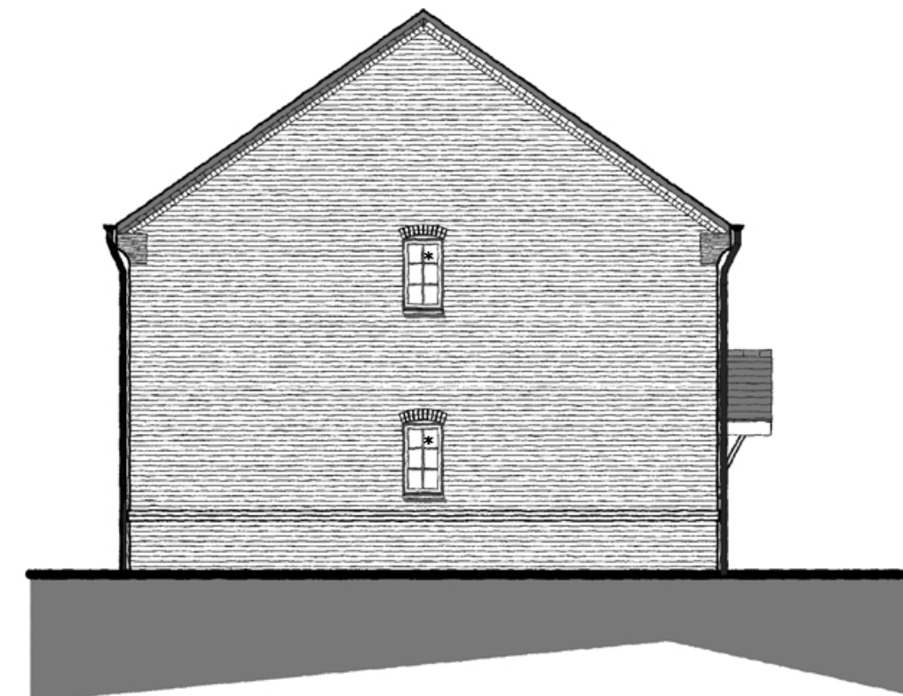
SIDE ELEVATION [2] - 1:100
