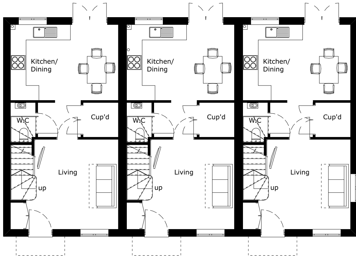
GROUND FLOOR - 1:100
