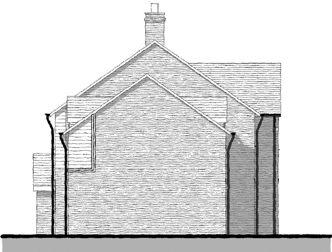
SIDE ELEVATION [2] - 1:100
