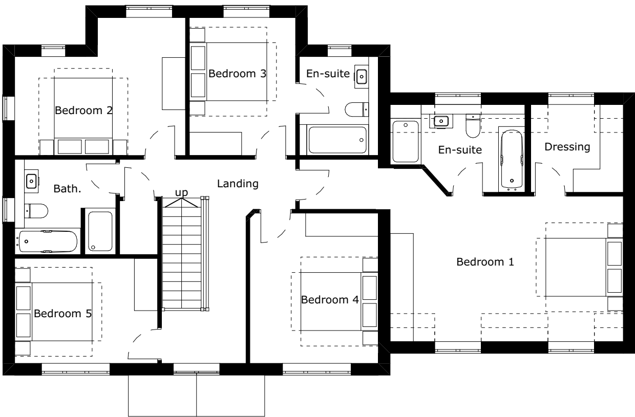
FIRST FLOOR - 1:100
