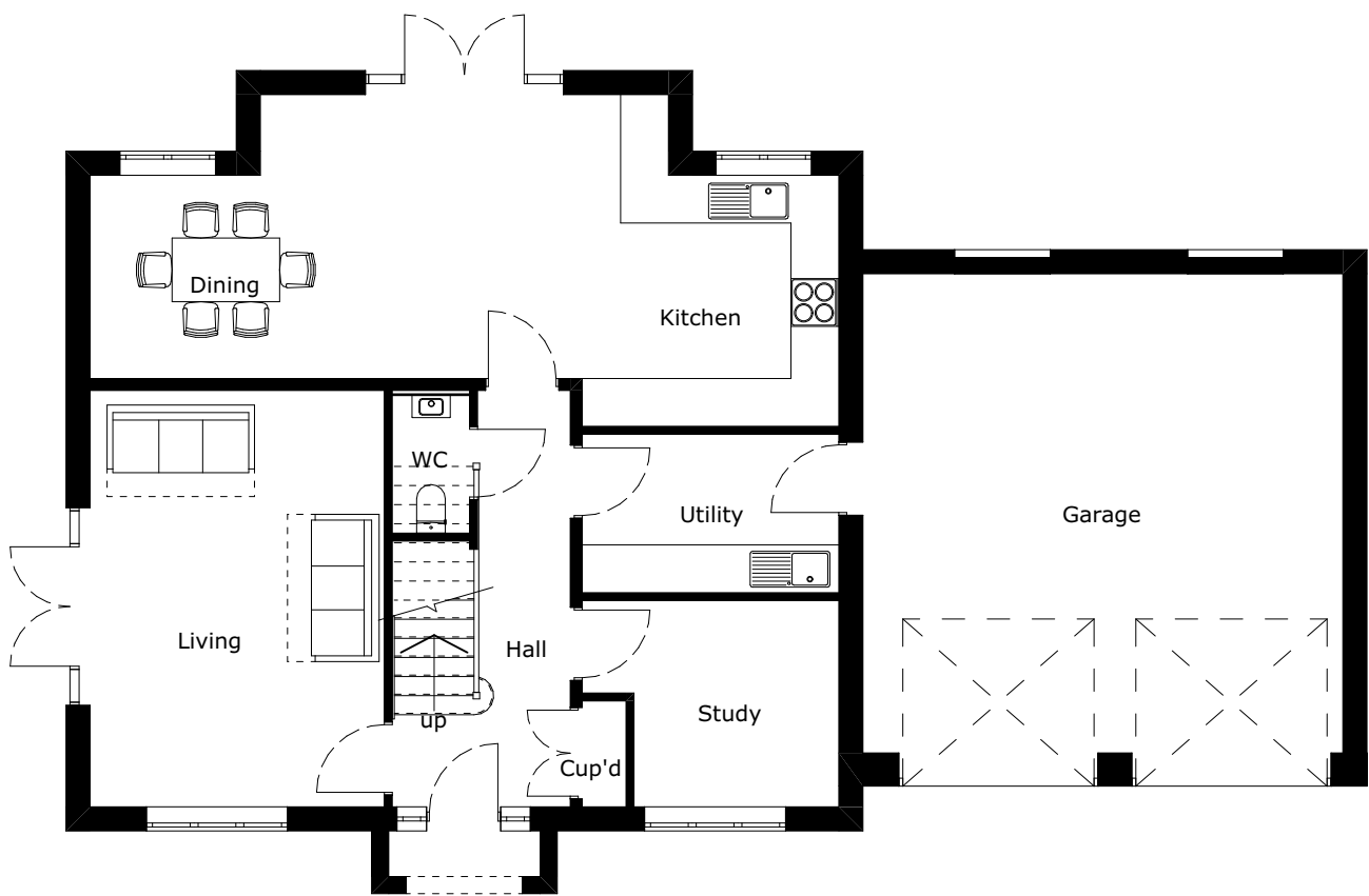
GROUND FLOOR - 1:100
