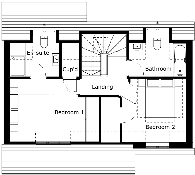
FIRST FLOOR - 1:100
