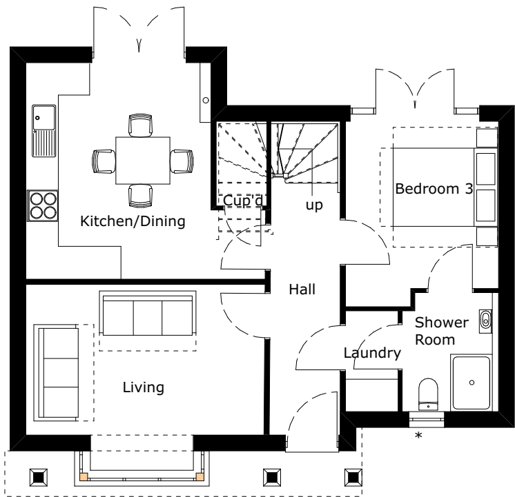
GROUND FLOOR - 1:100
