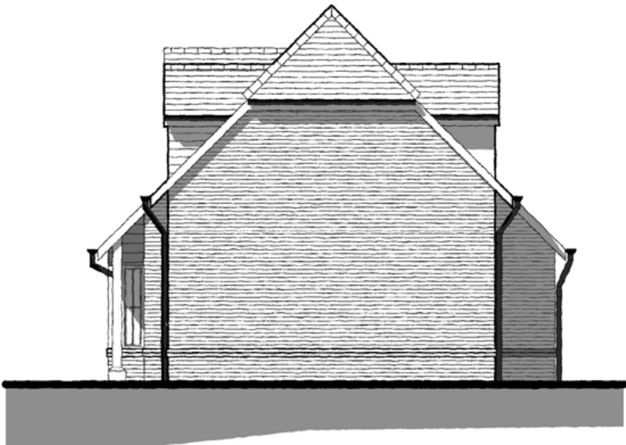
SIDE ELEVATION [2] - 1:100
