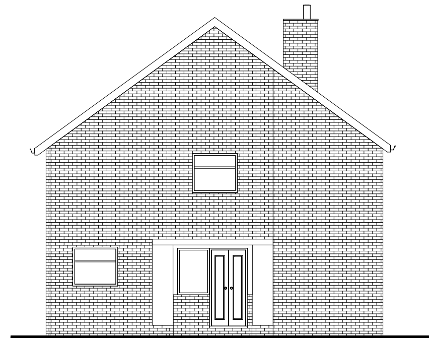
Existing NE Elevation
