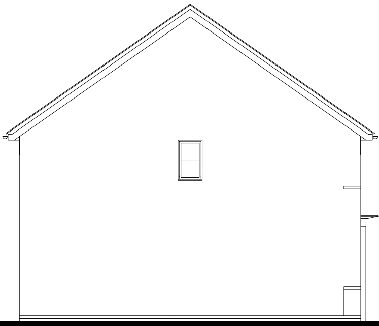
SIDE ELEVATION 1
