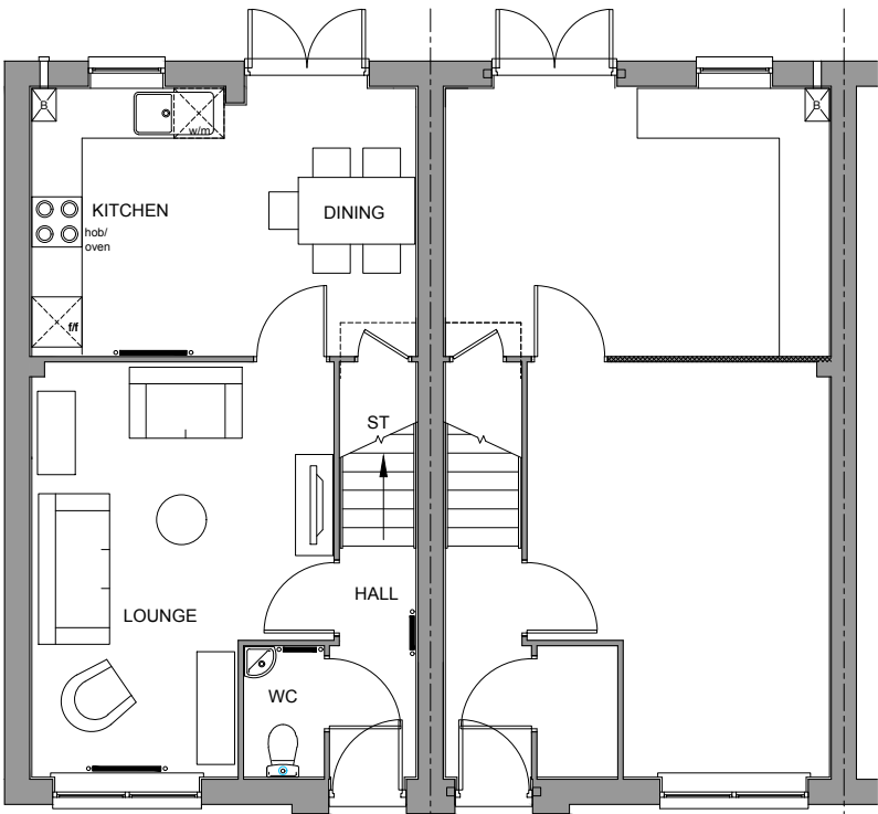
GROUND FLOOR PLAN MAIDSTONE
