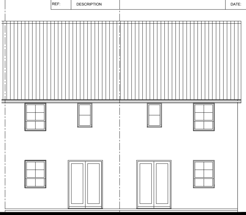
REAR ELEVATION
