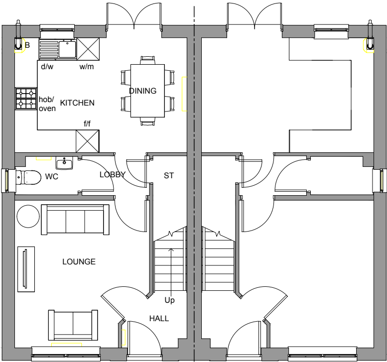
GROUND FLOOR PLAN ELLERTON
