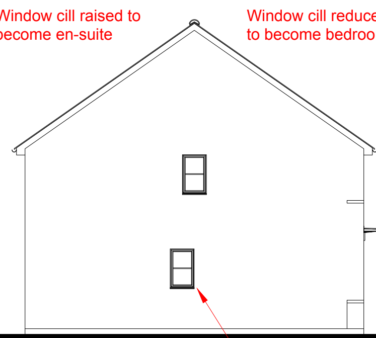
SIDE ELEVATION 1
