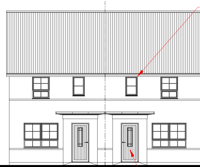
FRONT ELEVATION
