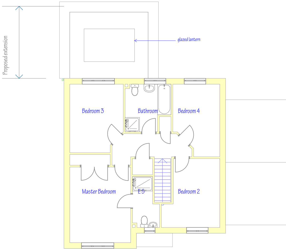
First Floor Plan as Proposed @ 1:100
