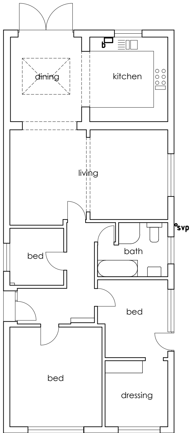
GROUND 1:100
