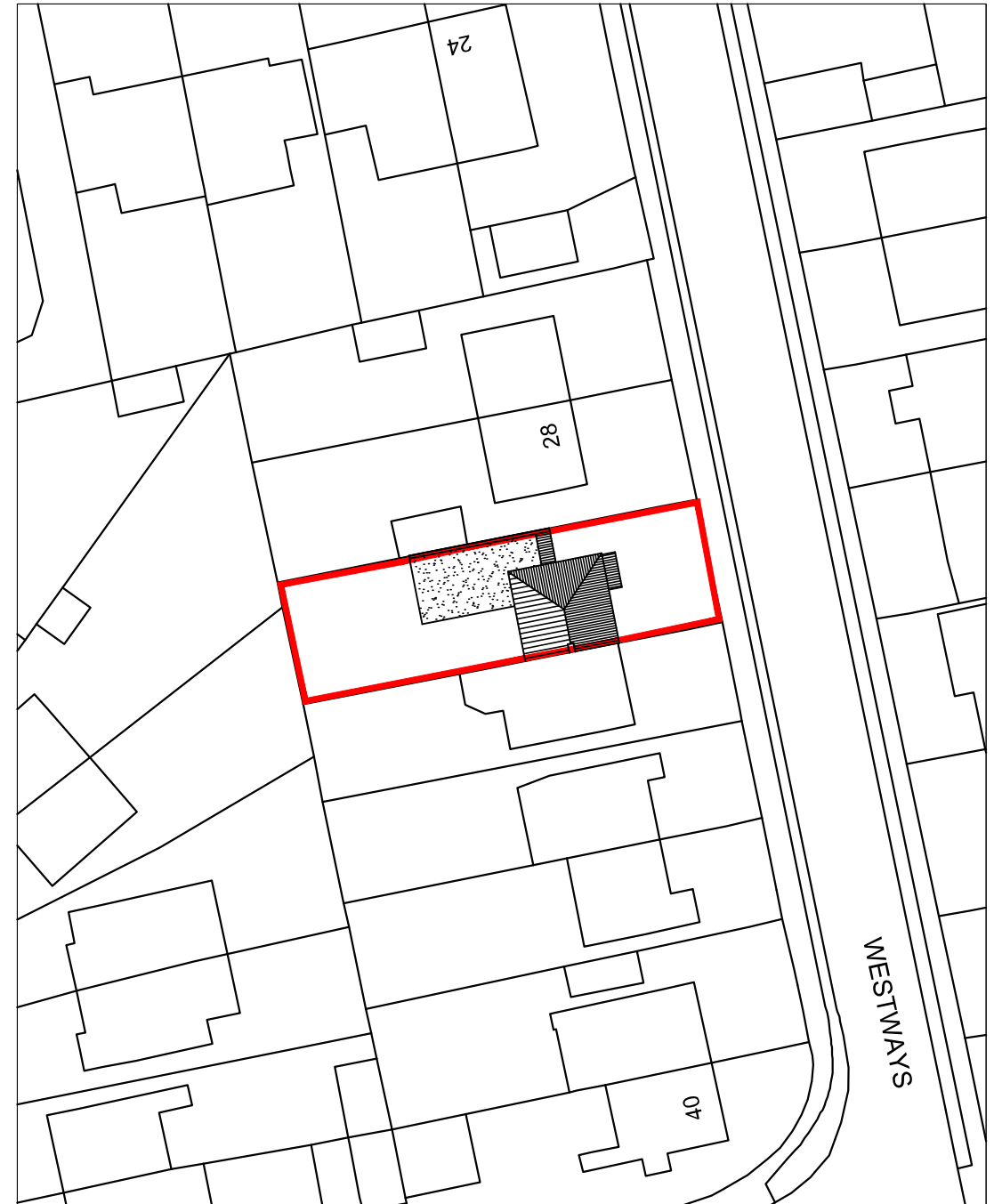
Block Plan: 1:500
