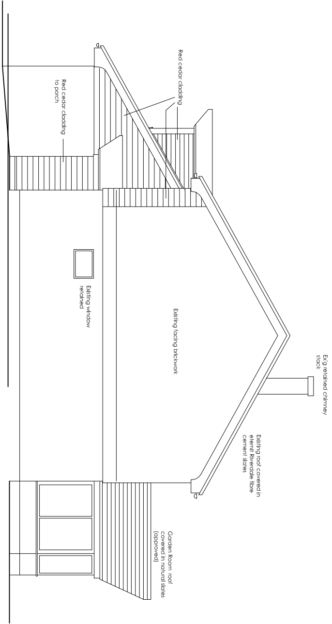
North Elevation
