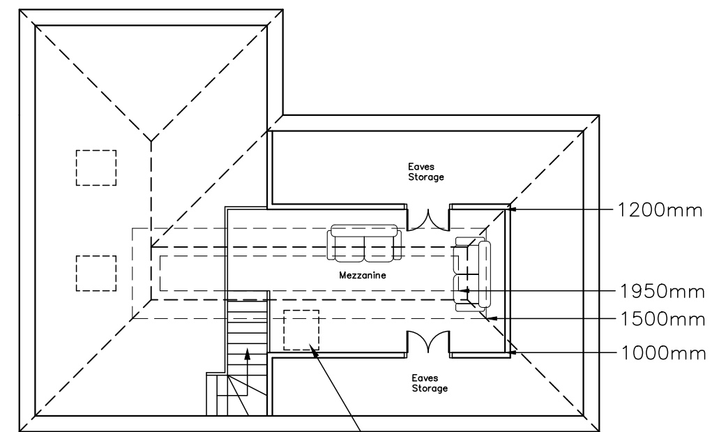
Mezzanine
