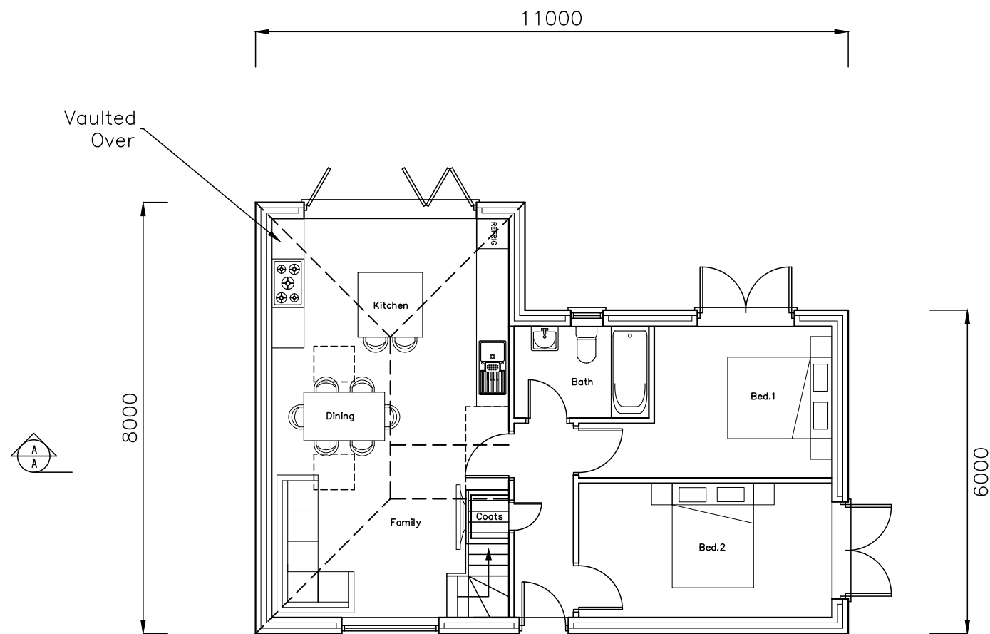
Ground Floor
