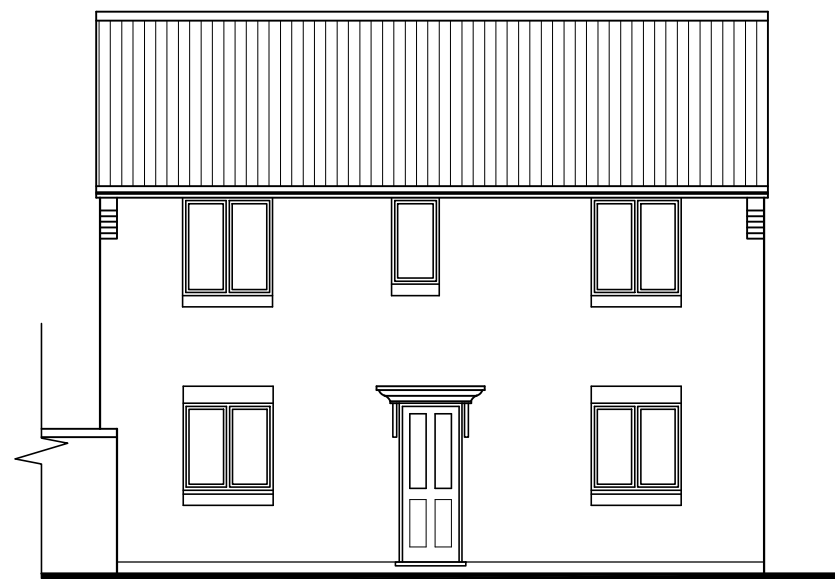
North
