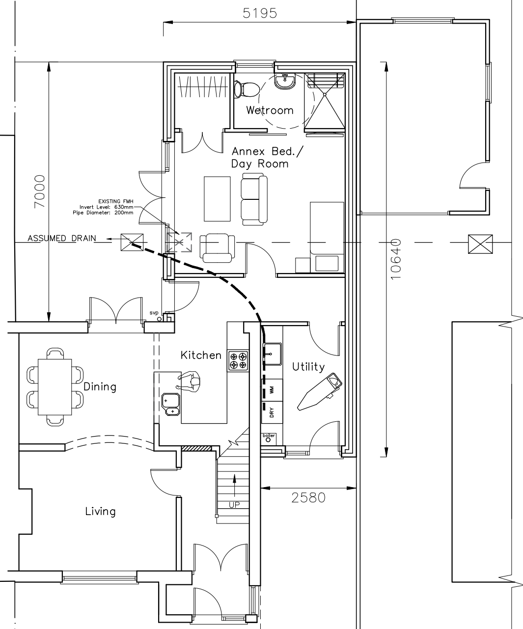
GROUND FLOOR
