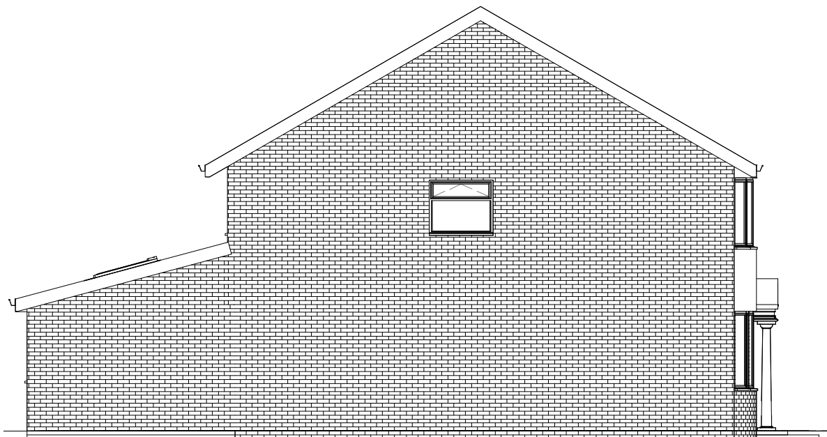
3 West Elevation 1 : 100
