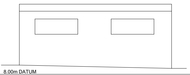
SOUTH ELEVATION
