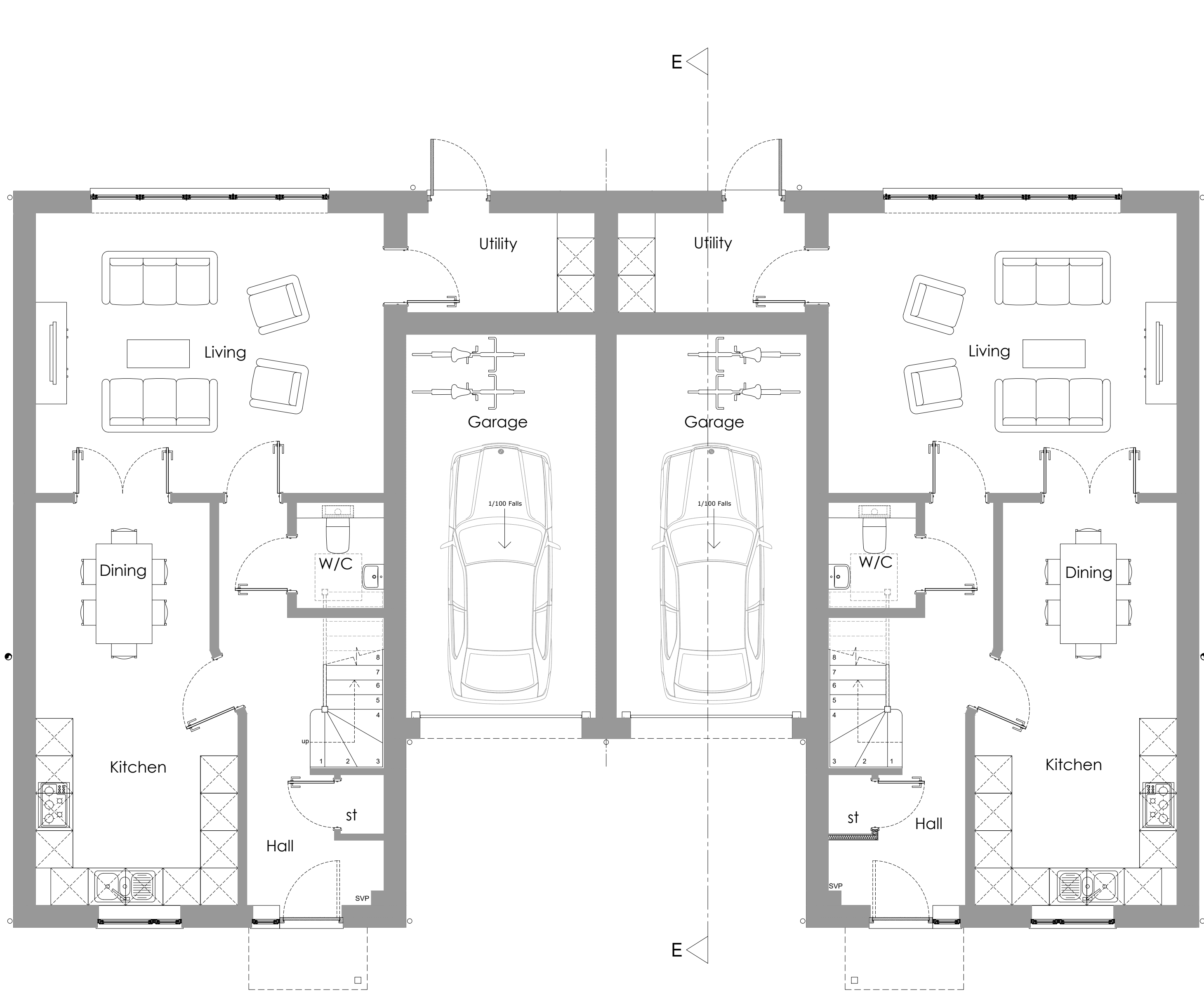
Approved Ground Floor Plan 1:50
