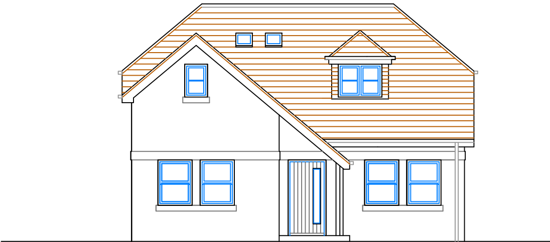
West Elevation
