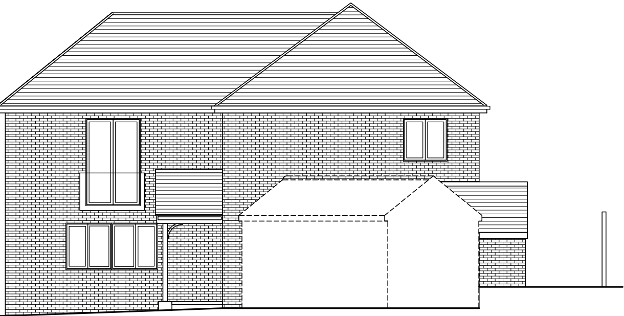
RIGHT FLANK ELEVATION 1:100 SCALE
