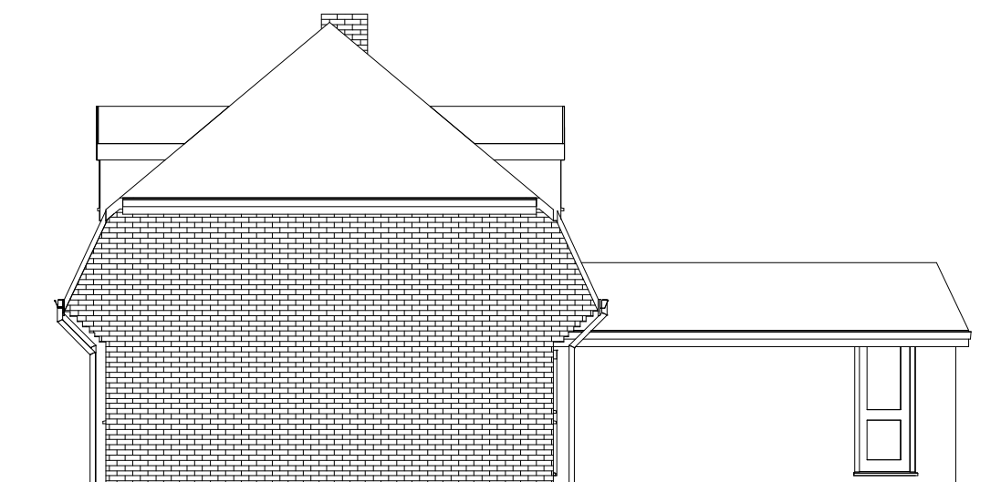
3 South Elevation 1 : 100
