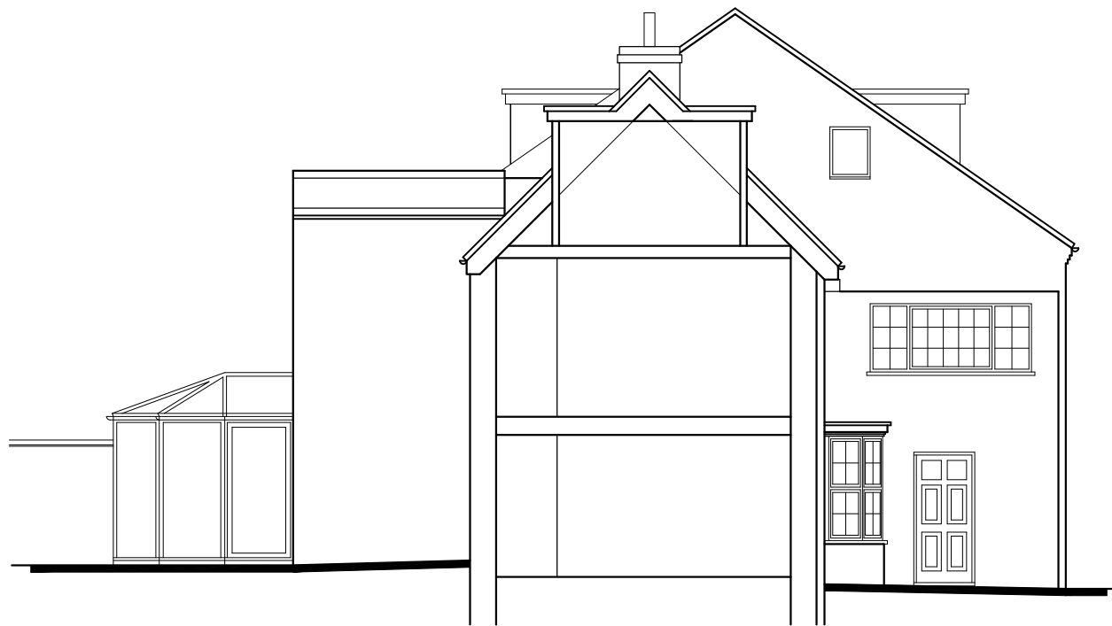
NORTH-WEST (PARTIAL SECTION)
