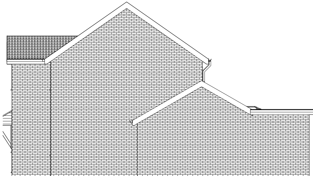
3 South Elevation 1 : 100
