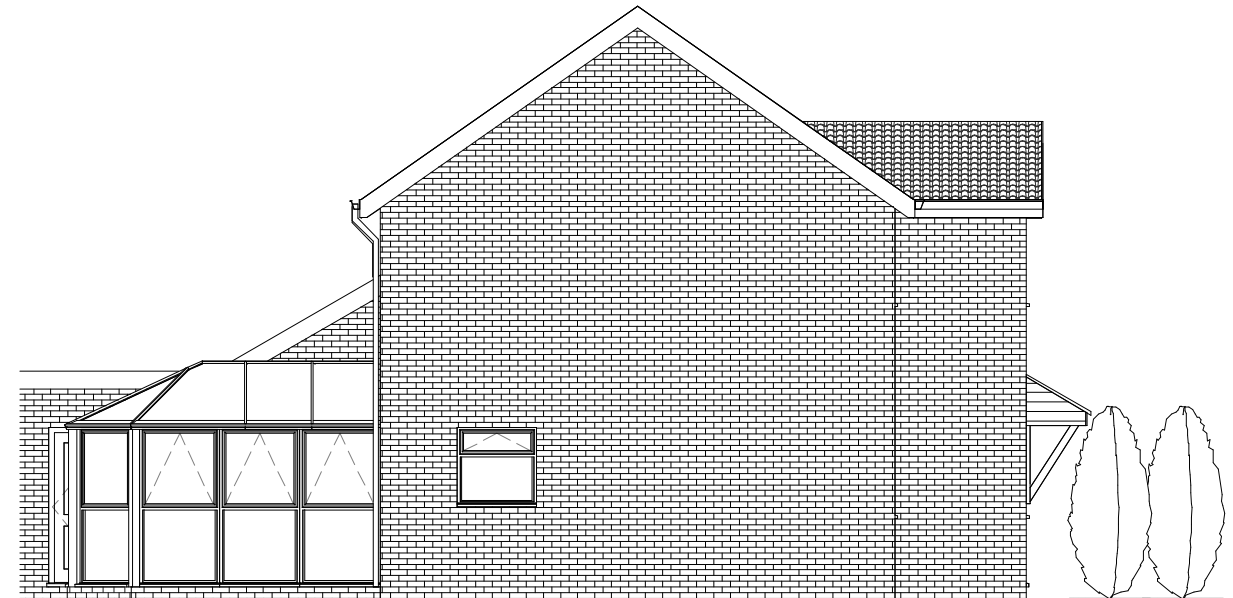
2 North Elevation 1 : 100
