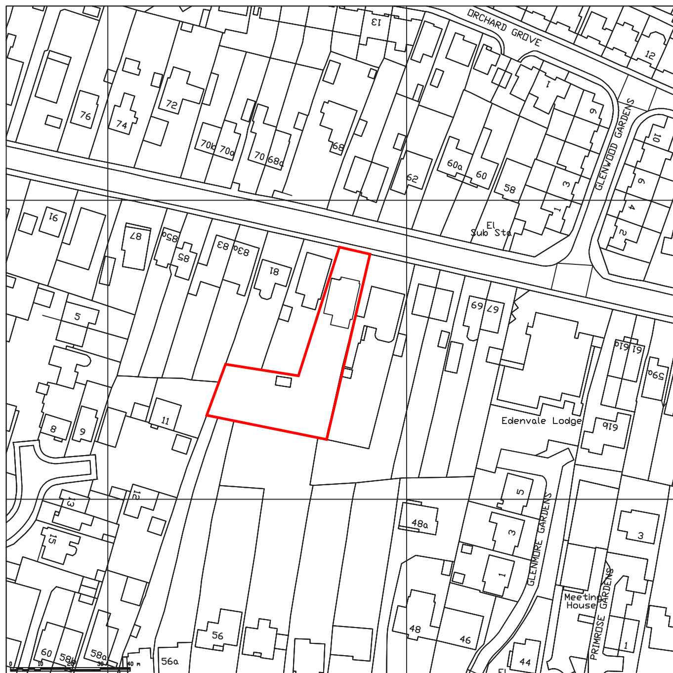
Site Plan @ 1:1250
