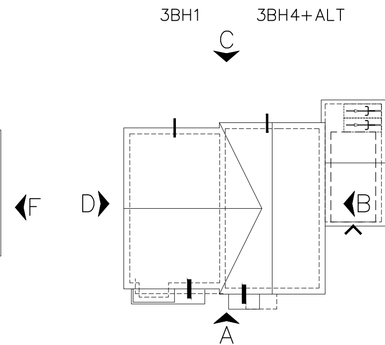
ROOF PLAN 1:200
