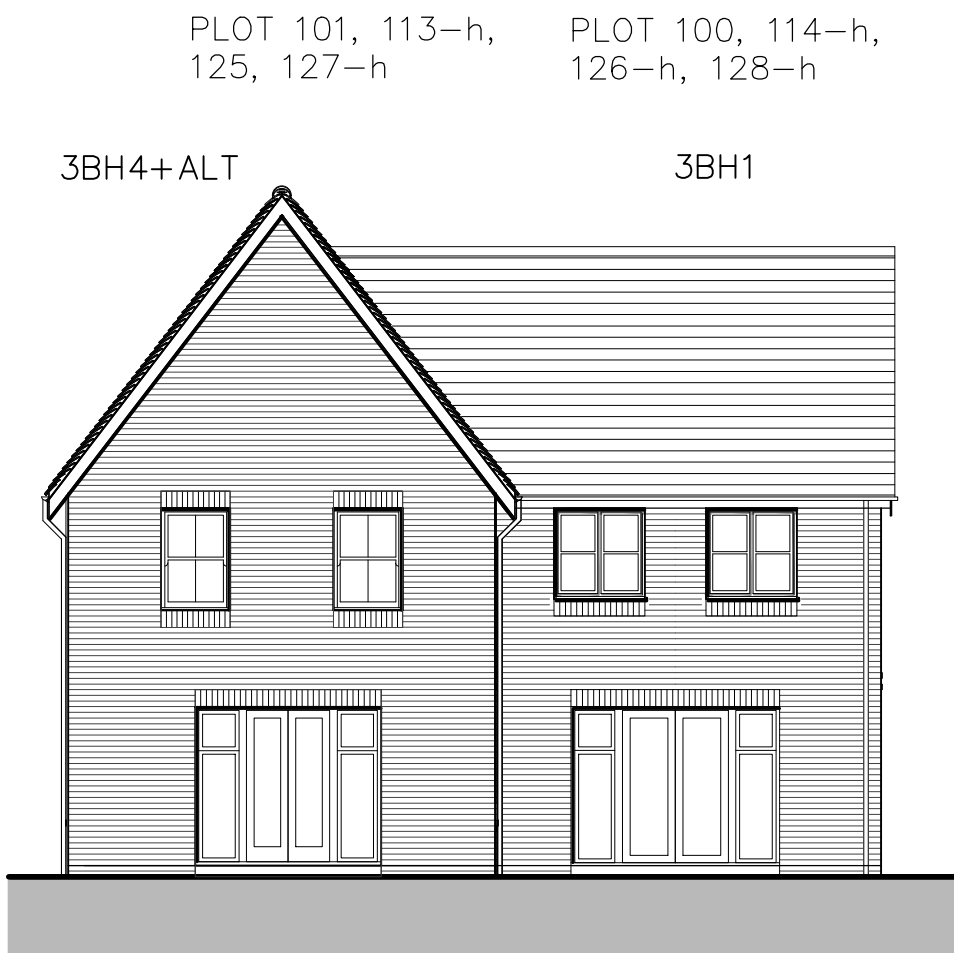
REAR ELEVATION – C
