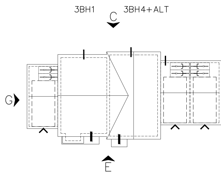
ROOF PLAN 1:200
