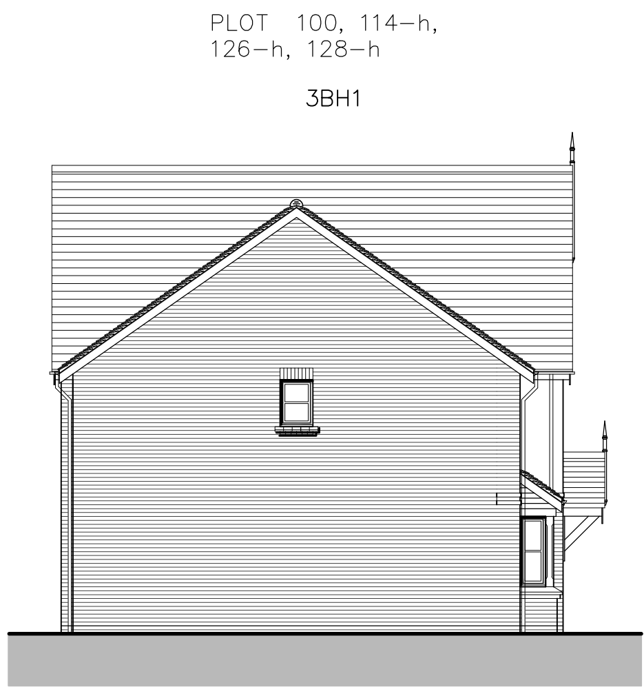
SIDE ELEVATION – D
