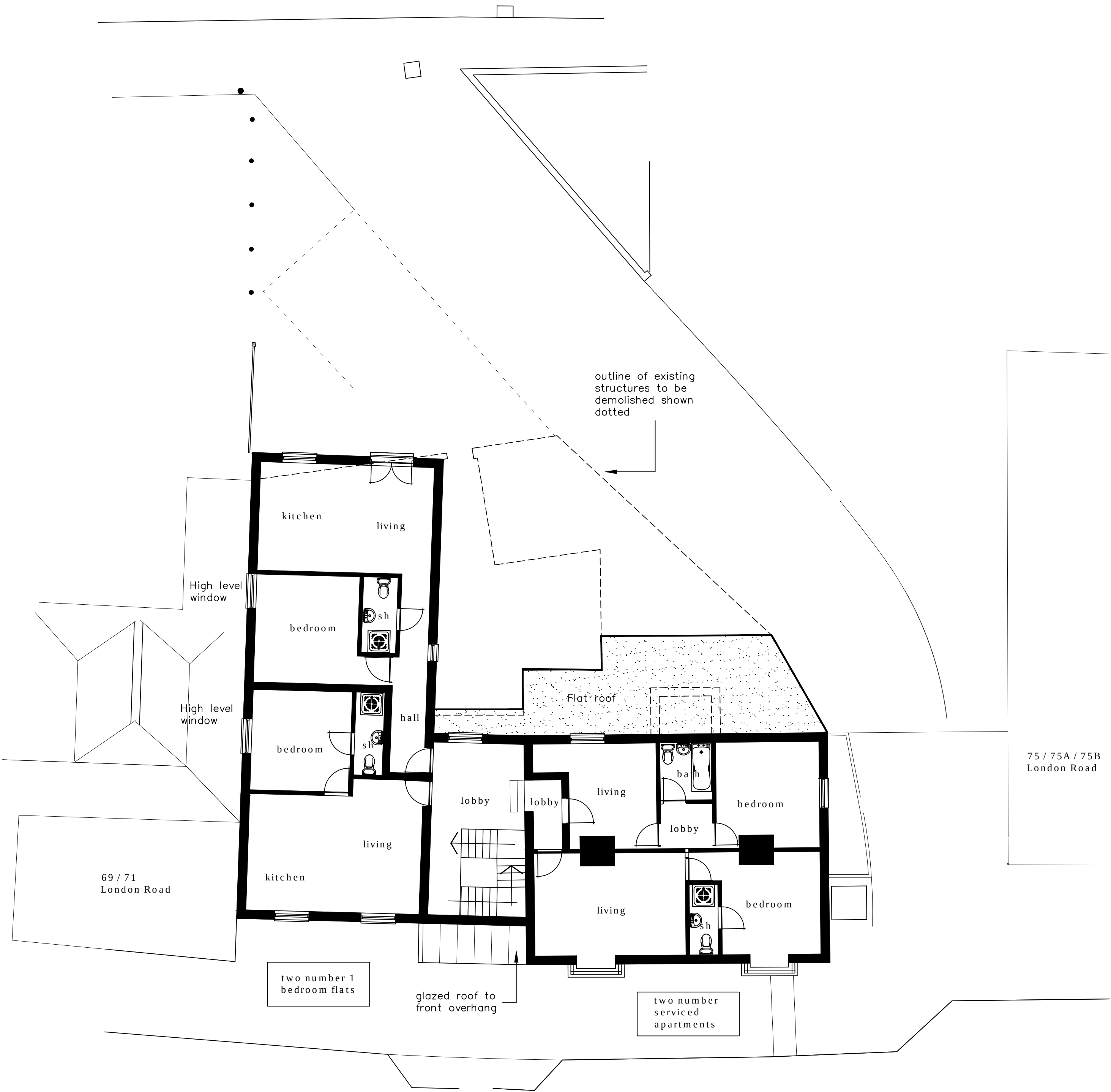
PROPOSED FIRST FLOOR SCALE 1:100
