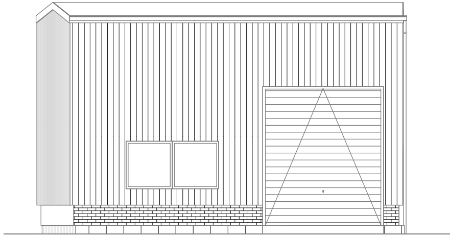
SOUTH ELEVATION 1 : 100
