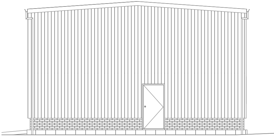
EAST ELEVATION 1 : 100
