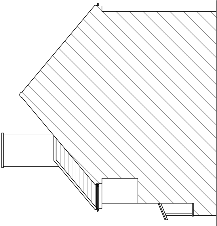
EXISTING SIDE ELEVATION / SECTION
