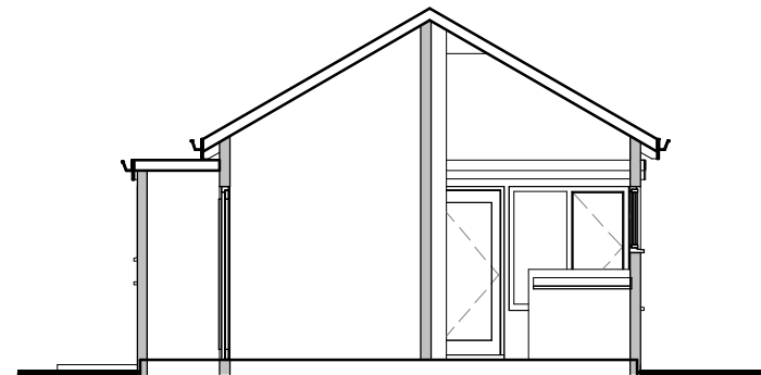
1 East west site section 1 : 100
