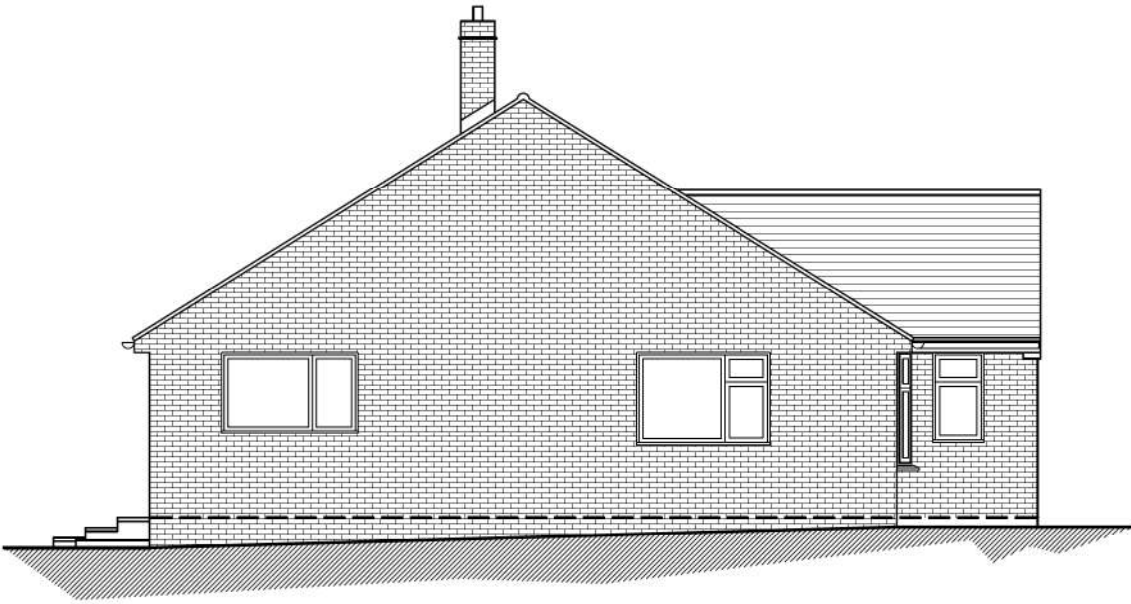
RIGHT ELEVATION 1:100 SCALE
