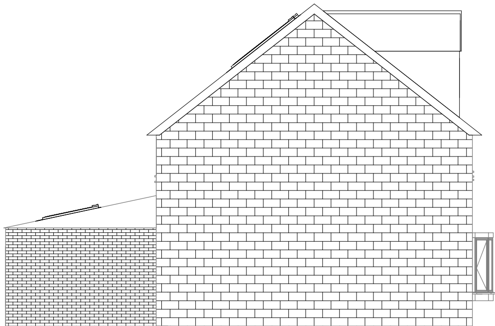
WP West Proposed 1 : 100
