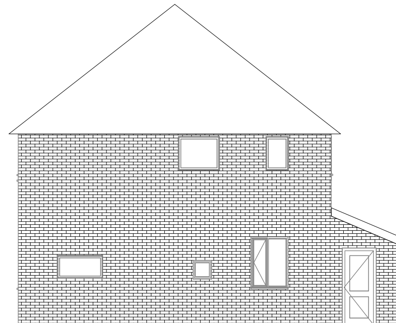
EE East Existing 1 : 100
