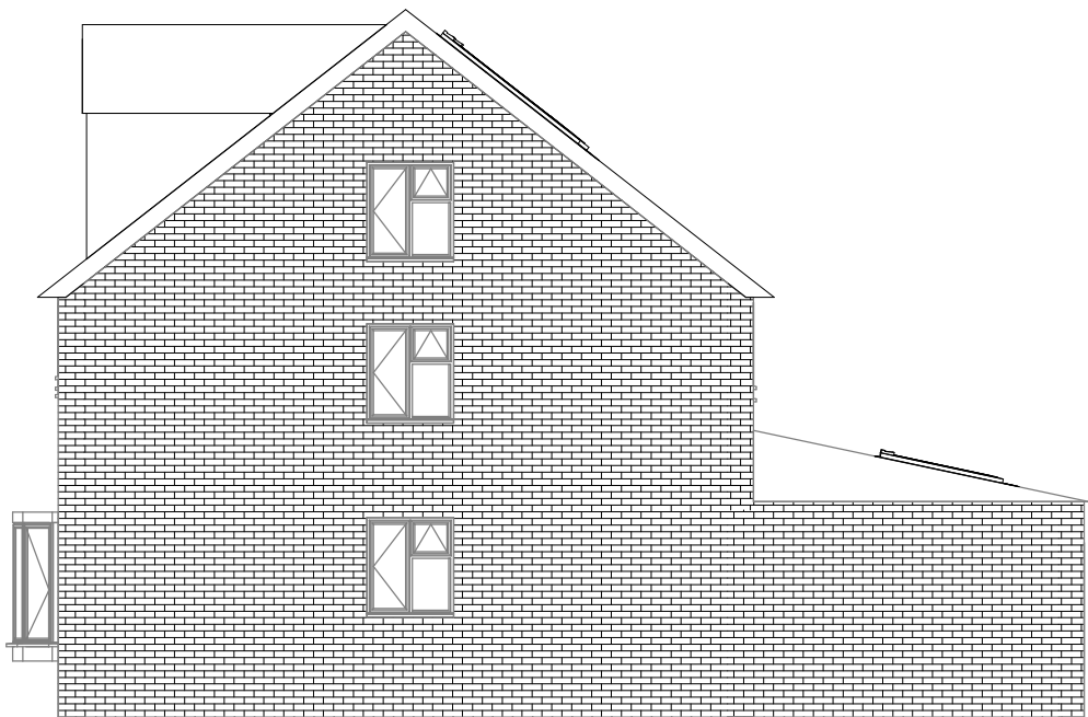
EP East Proposed 1 : 100
