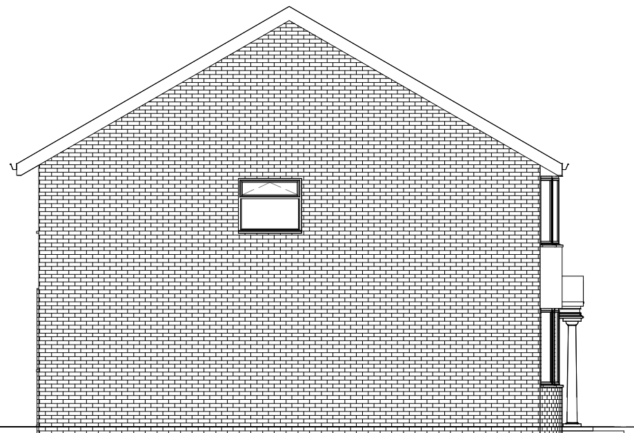
3 West Elevation 1 : 100
