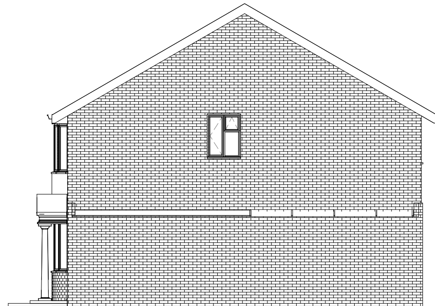
2 East Elevation 1 : 100
