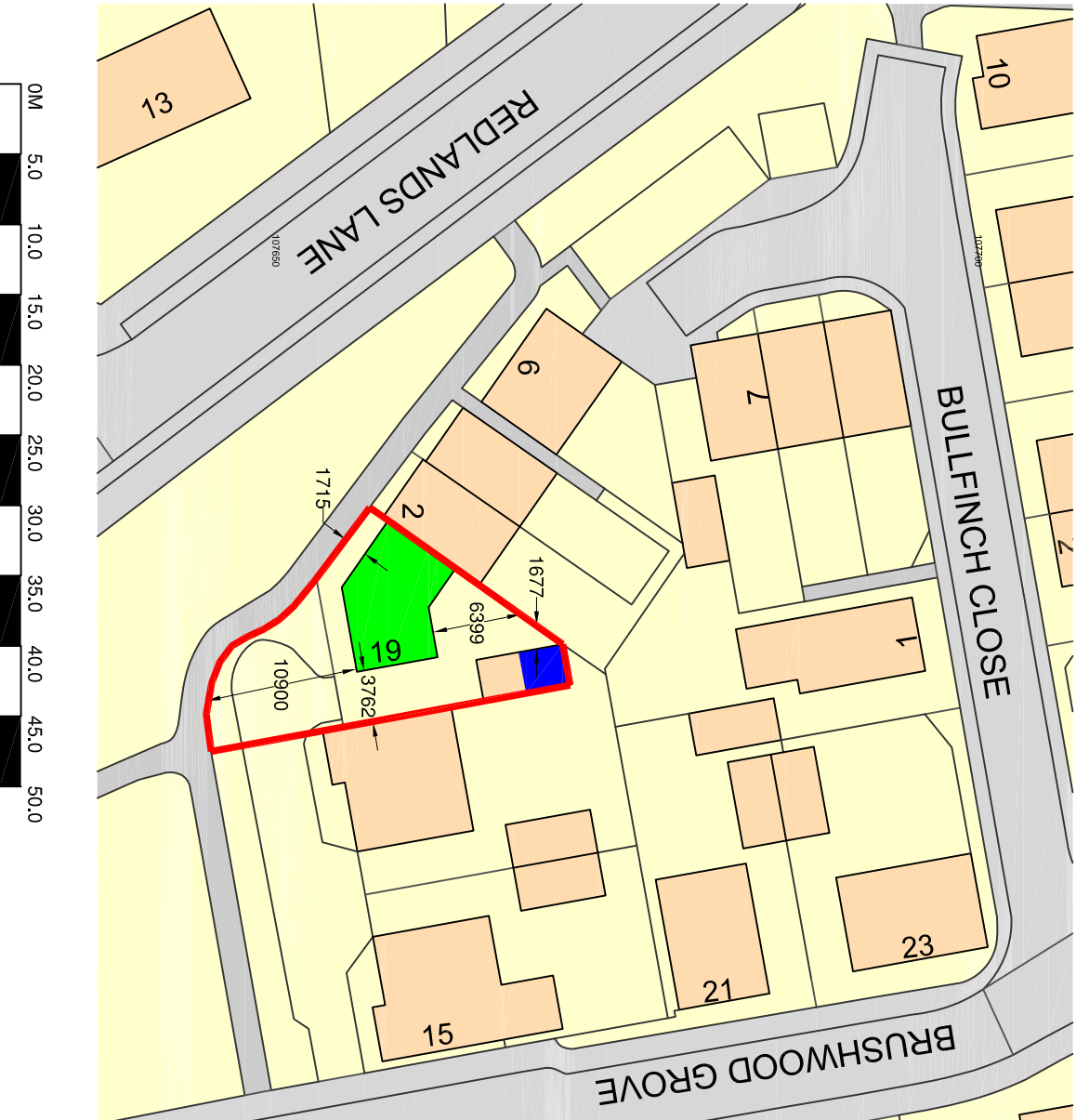
Site Plan at 1:500 Scale
