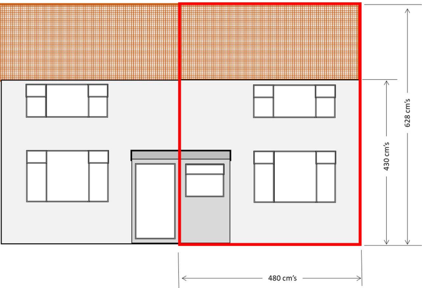
Front (South) Elevation
