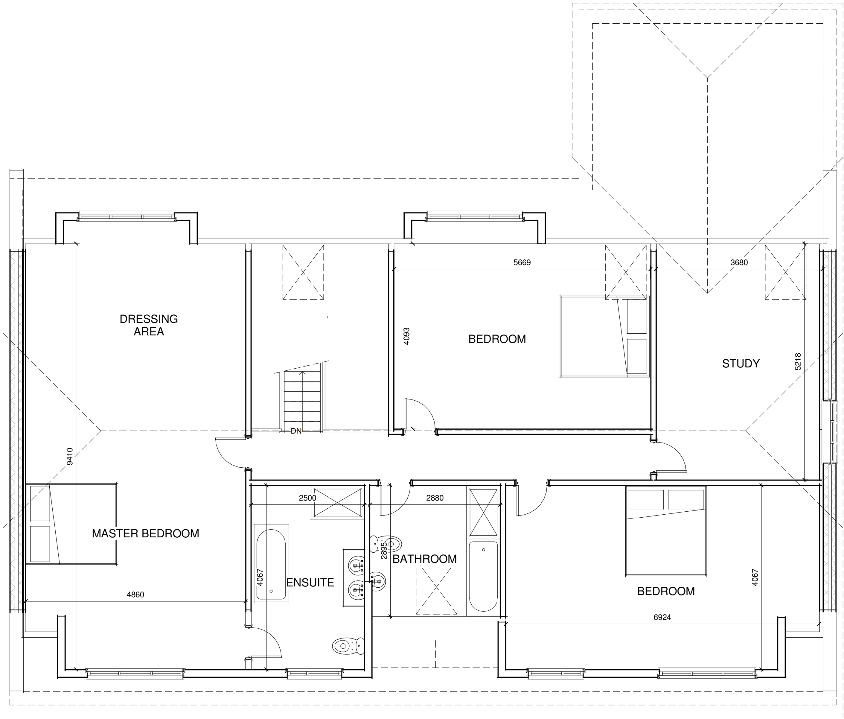
Proposed First Floor 1 : 50
