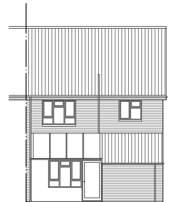
South Elevation
