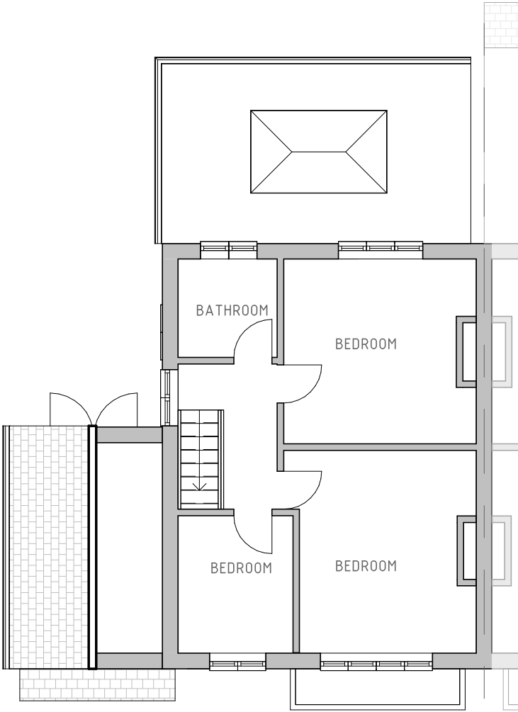
03/102 - EXISTING FIRST FLOOR PLAN 1 : 100
