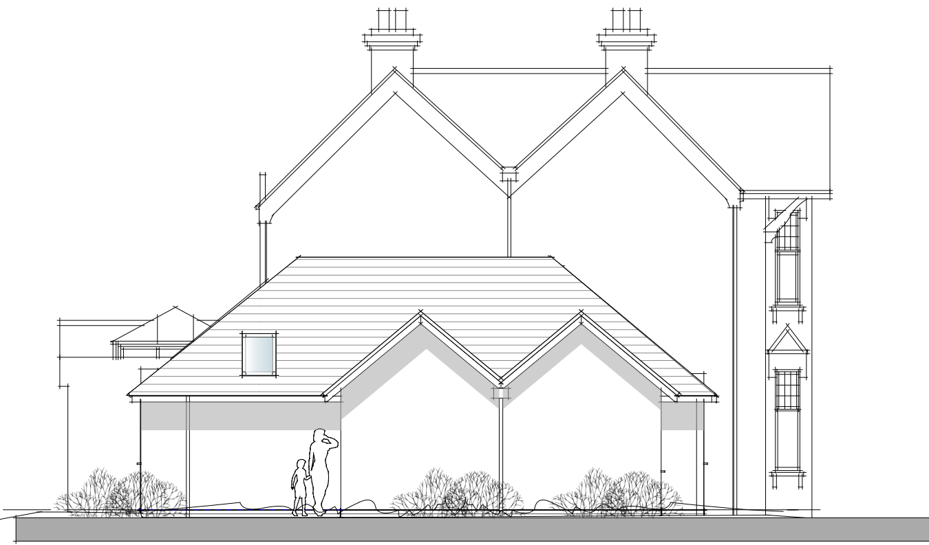
NORTH ELEVATION
