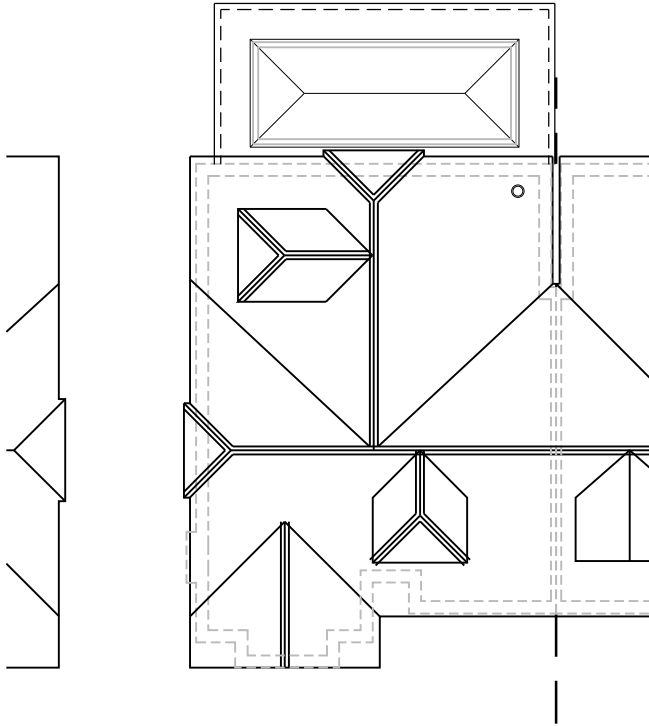
Roof Plan
