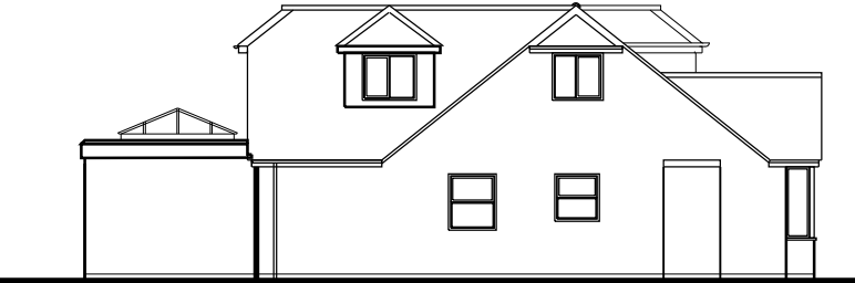
West Elevation
