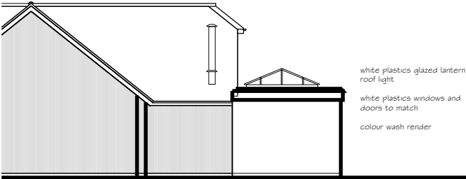
East Elevation
