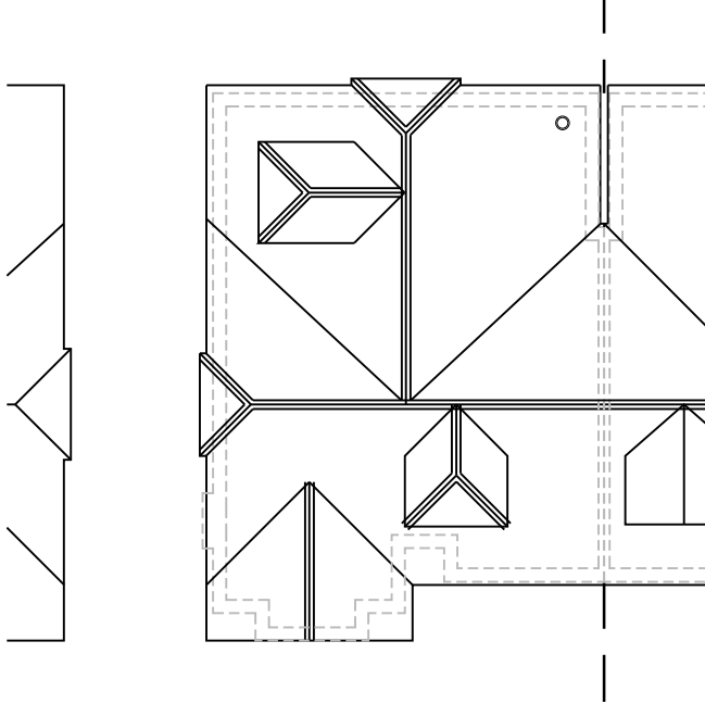
Roof Plan
