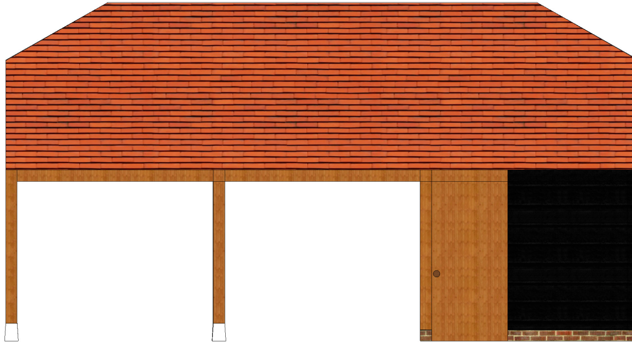
Proposed garage at the Old Workshop North Elevation (as viewed from garden) Scale 1:50 at A4
