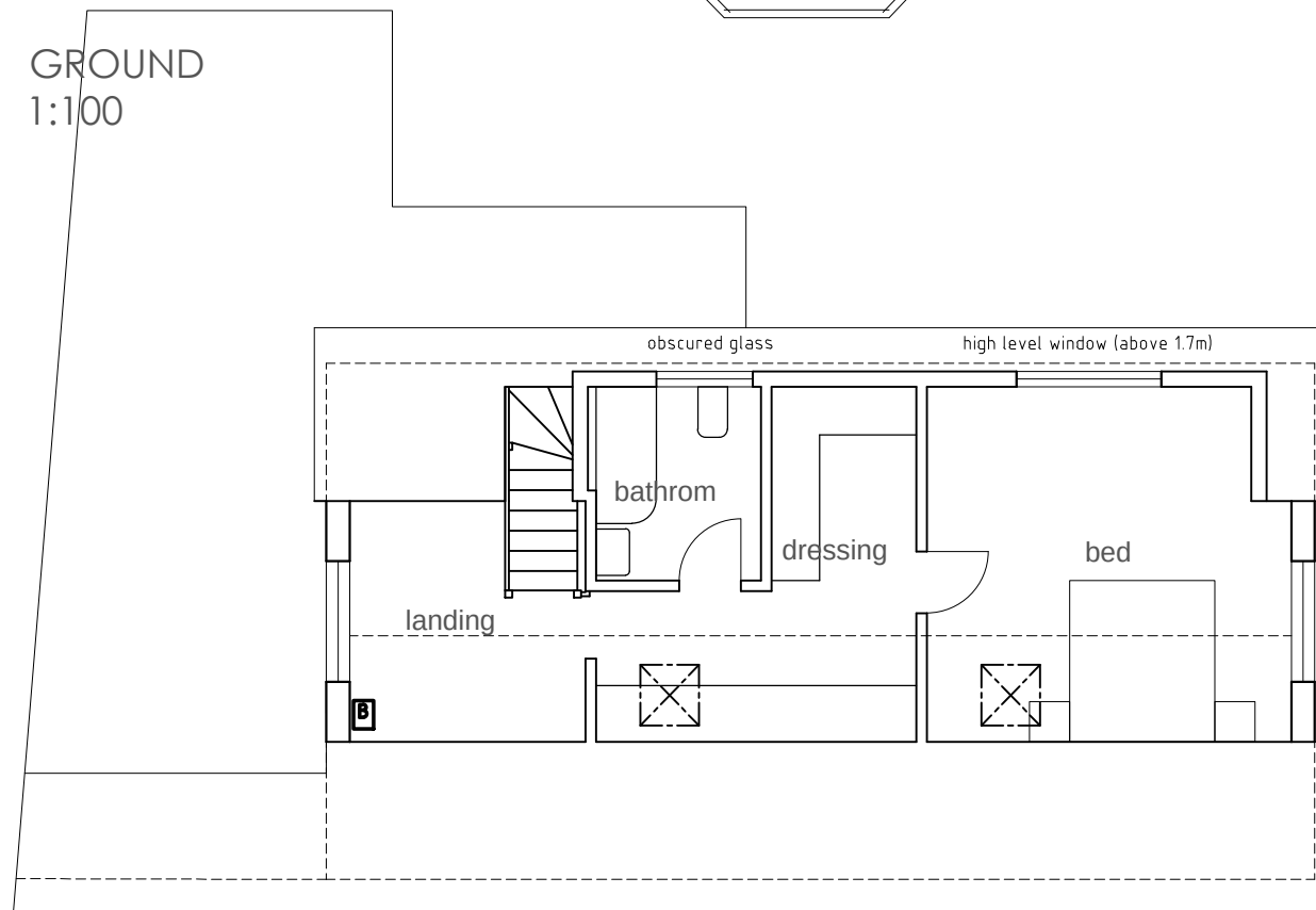
FIRST 1:100
