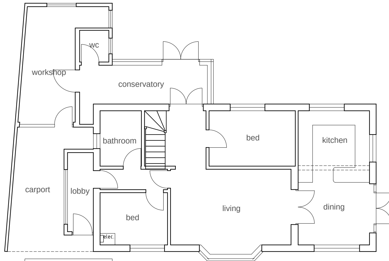
GROUND 1:100
