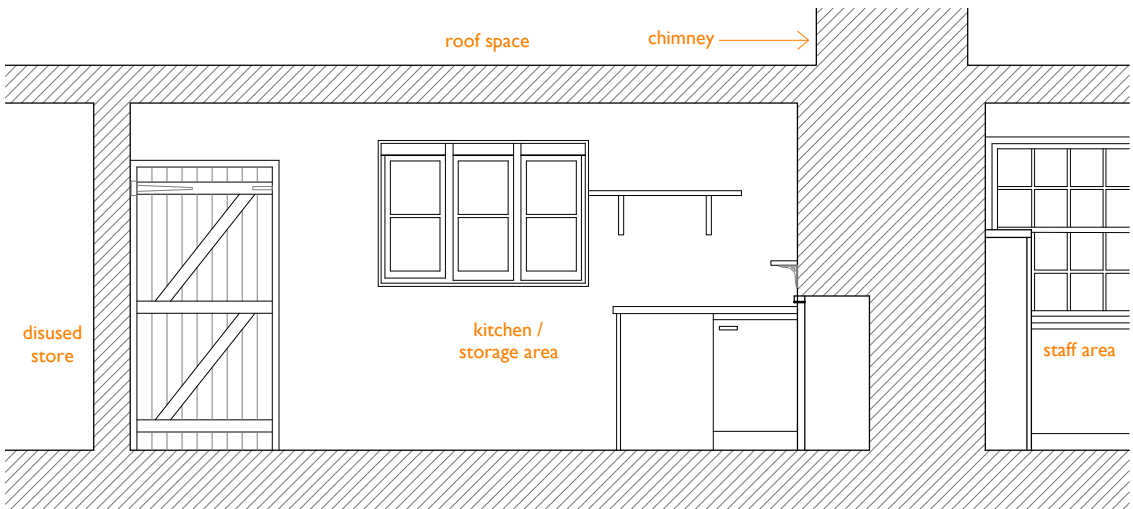
EXISTING SECTION K-K 1:50
