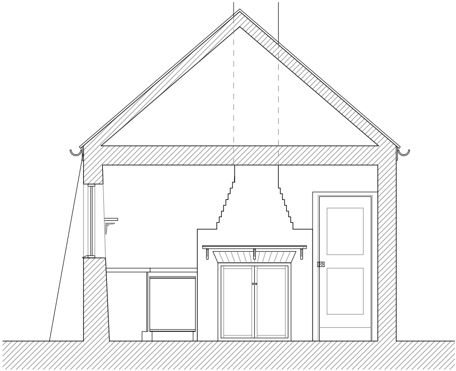
EXISTING SECTION H-H 1:50
