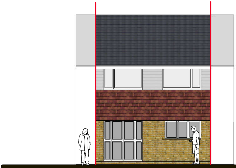
A 3 Rear Elevation 1:100
