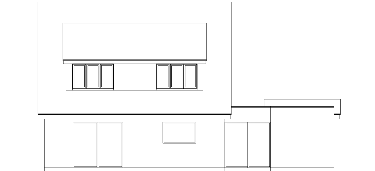
South Elevation | Existing
