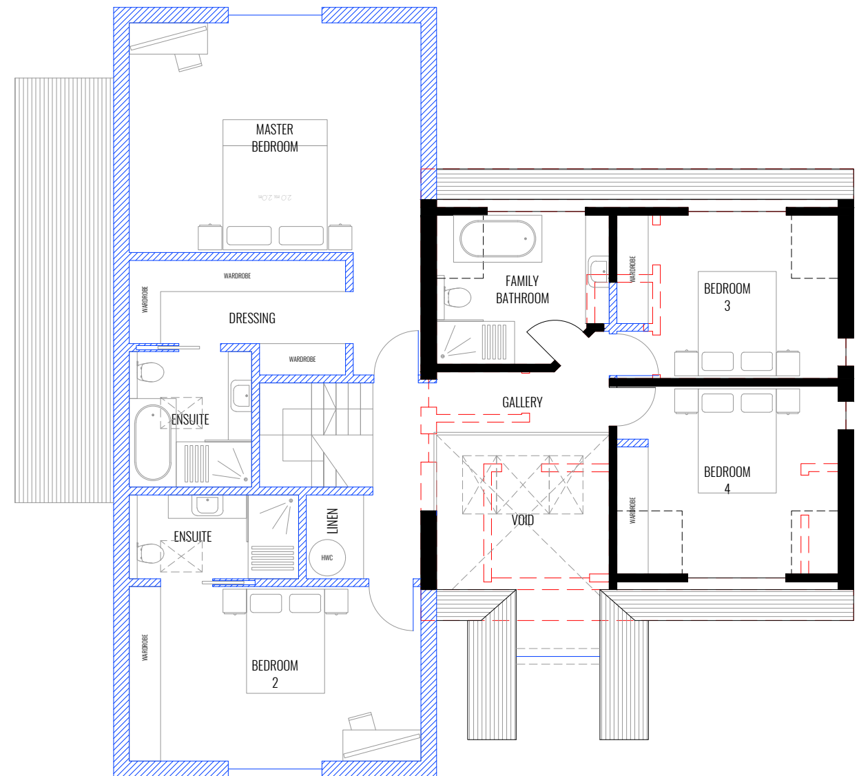
First Floor Plan | Proposed
