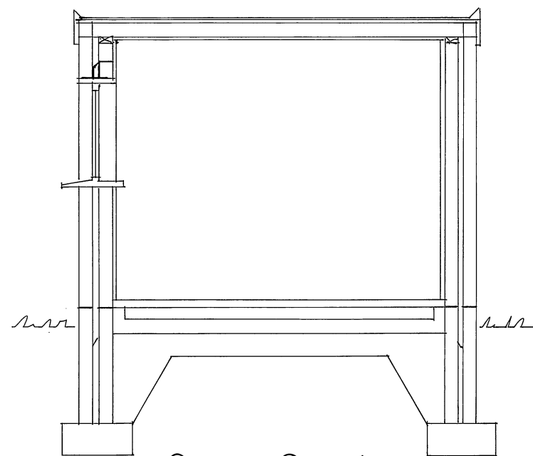
Cross-Section
