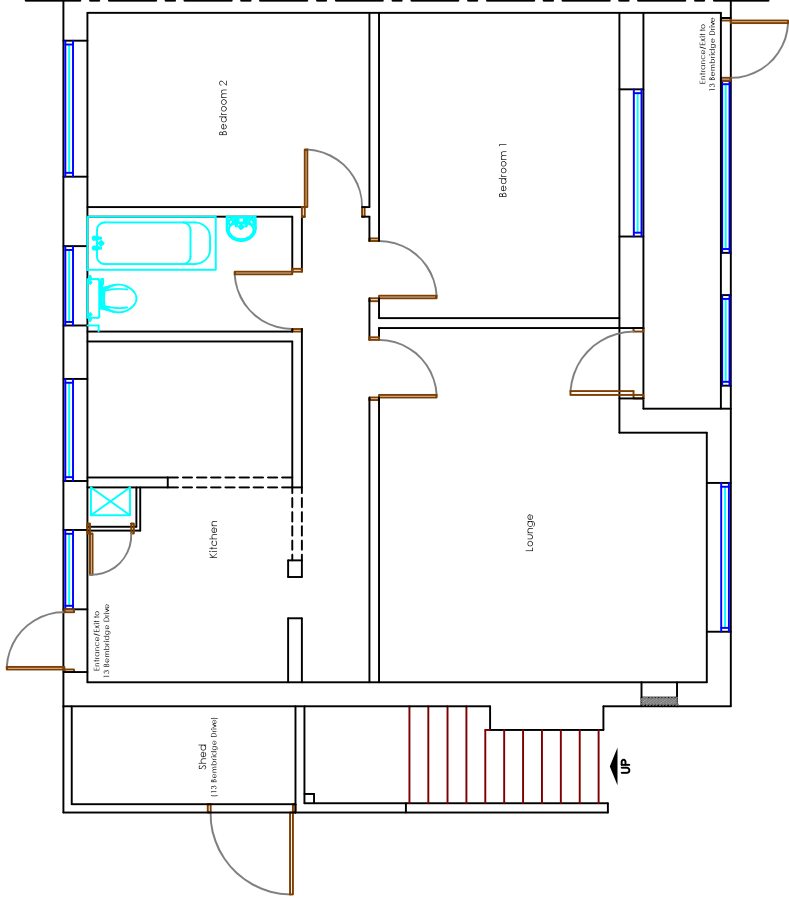
PROPOSED GROUND FLOOR (13 Bembridge Drive) - No changes
