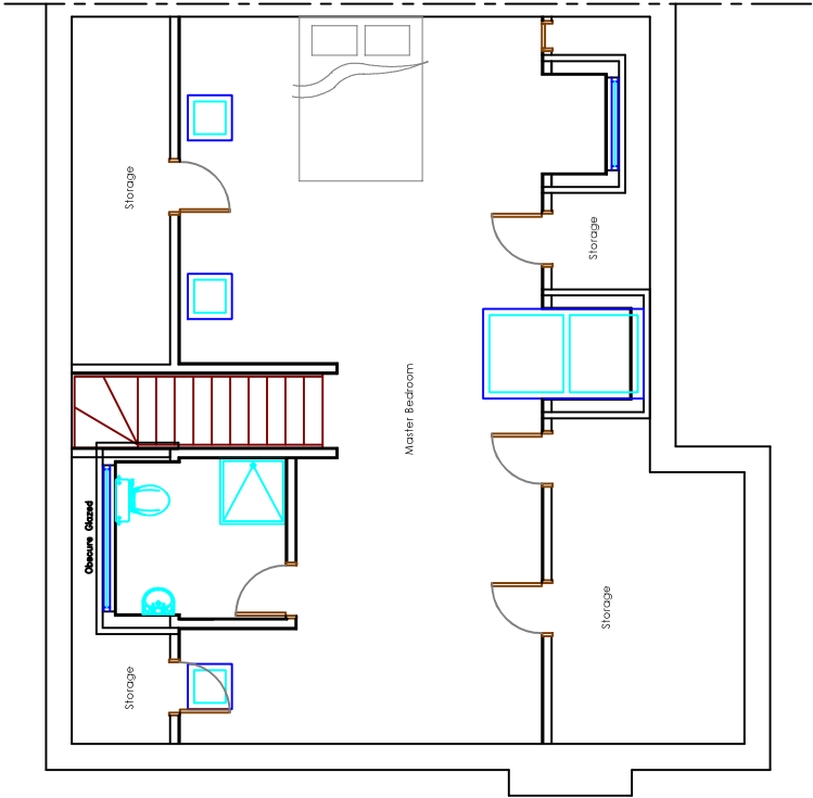
PROPOSED LOFT / 2ND FLOOR (13A Bembridge Drive)
