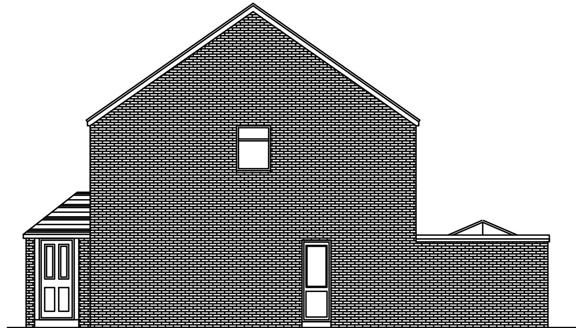
Proposed side elevation (Garage removed for clarity)
