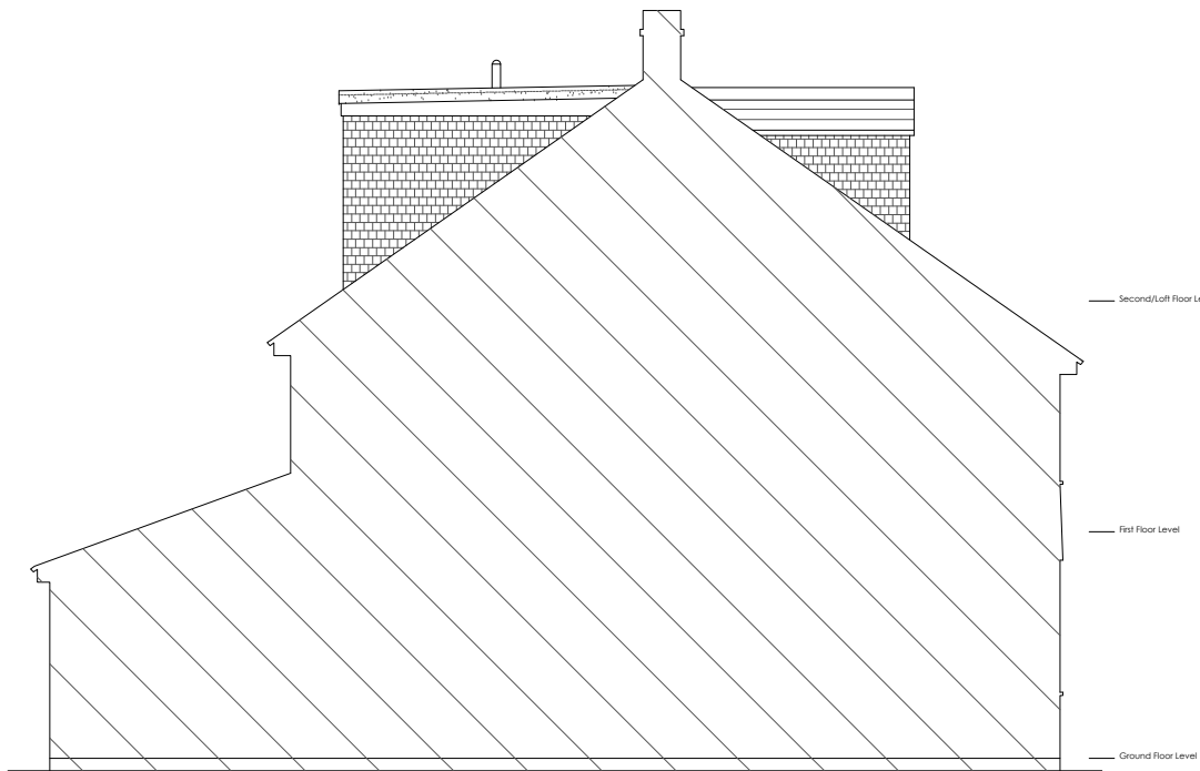
PROPOSED SIDE SECTION/ELEVATION
