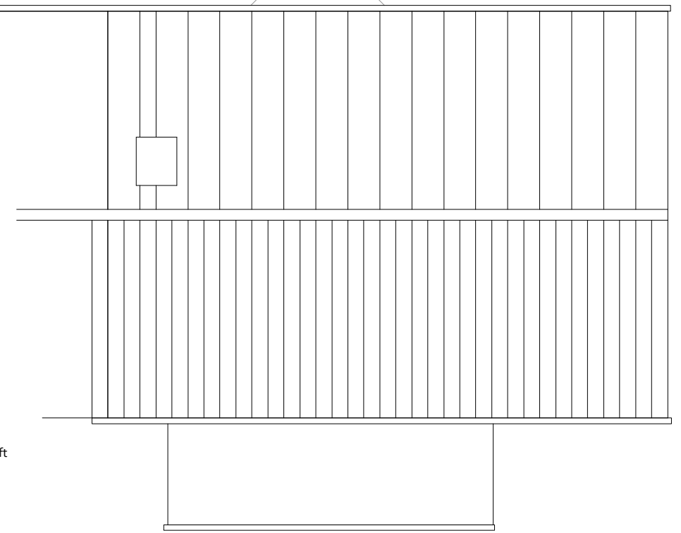
Roof plan
