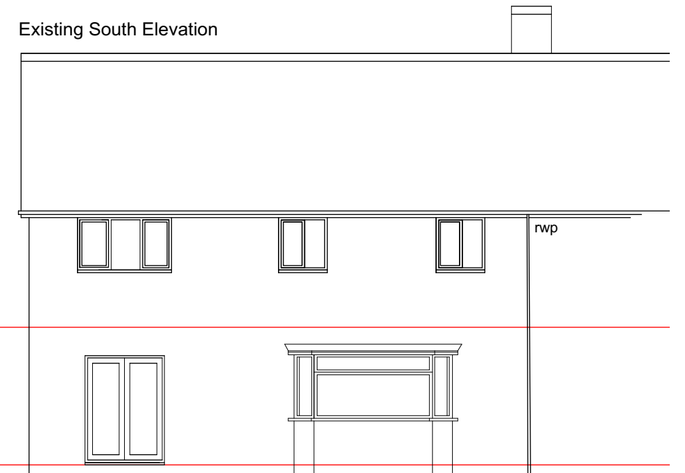
1. Existing plans & Elevations : Scale 1 - 100@A3
